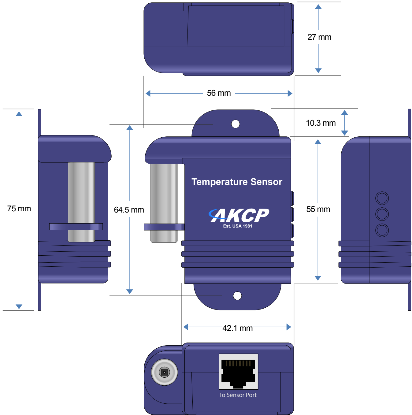
TMP00 - Extendable Temperature Sensor
